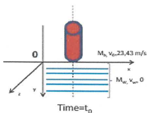
Figure 2. Water impact
